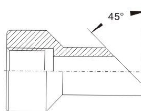
45° 直形连接接头 Straight union joint
