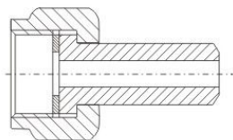
压力表接头 Pressure gauge joint
