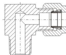
(卡套式)弯通接头 (Ferrule) Goose-neck joint
