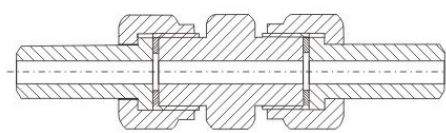
对焊式直通终端接头 Butt-welding straight-in terminal joint
