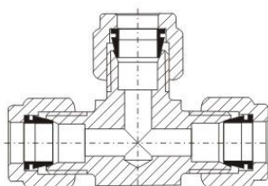
(卡套式)三通终端接头 (Ferrule) T-cock terminal joint
