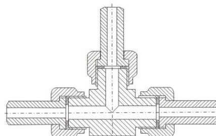
三通中间接头 T-cock intermediate joint
