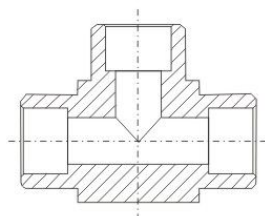
三通承插焊接头 T-cock socket weld joint
